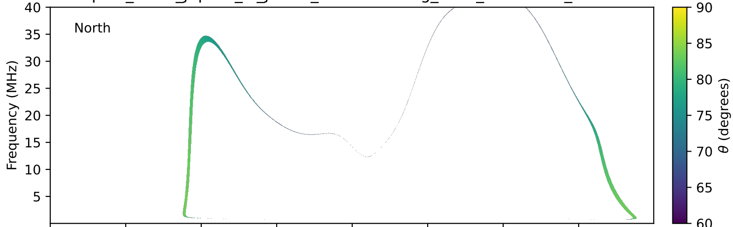
expres_earth_jupiter_io_jrm33_lossc-wid1deg_3kev_20281109_v11.cdf
