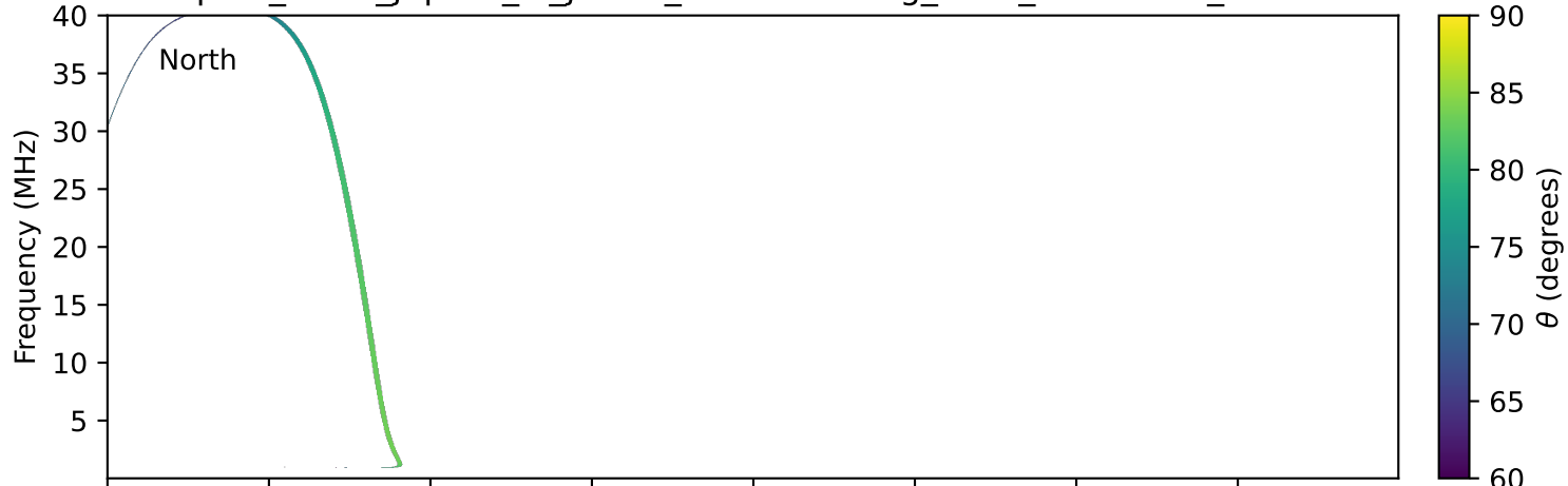
expres_earth_jupiter_io_jrm33_lossc-wid1deg_3kev_20281108_v11.cdf
