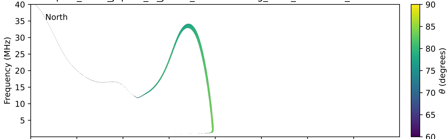
expres_earth_jupiter_io_jrm33_lossc-wid1deg_3kev_20281106_v11.cdf
