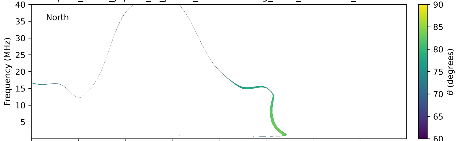
expres_earth_jupiter_io_jrm33_lossc-wid1deg_3kev_20281104_v11.cdf
