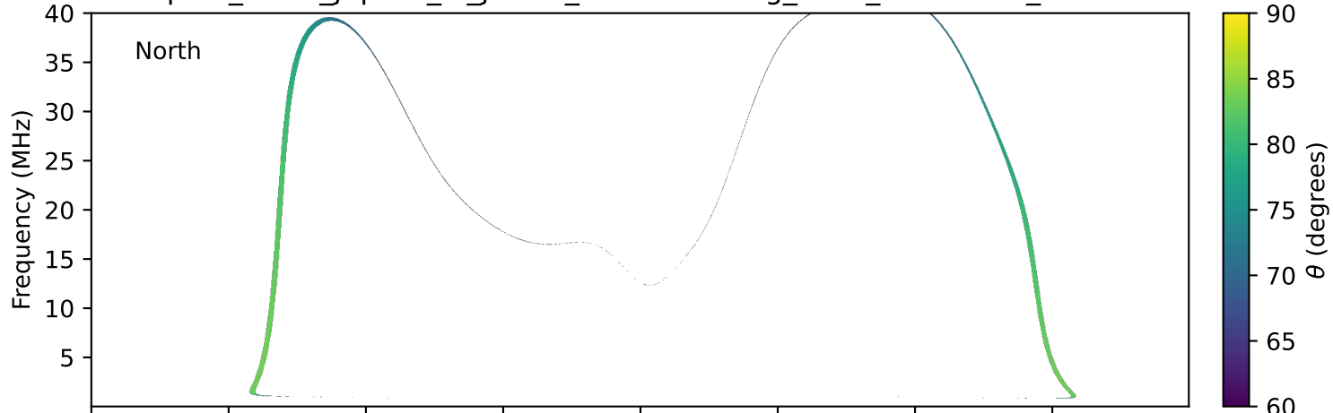
expres_earth_jupiter_io_jrm33_lossc-wid1deg_3kev_20281102_v11.cdf
