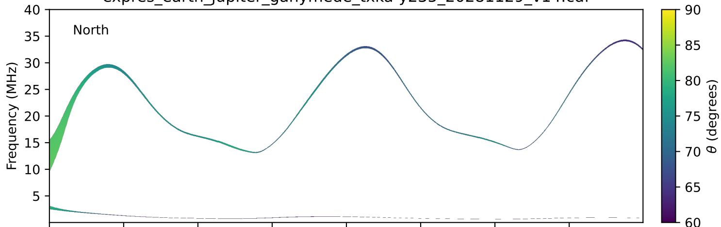
expres_earth_jupiter_ganymede_txka-y235_20281129_v14.cdf
