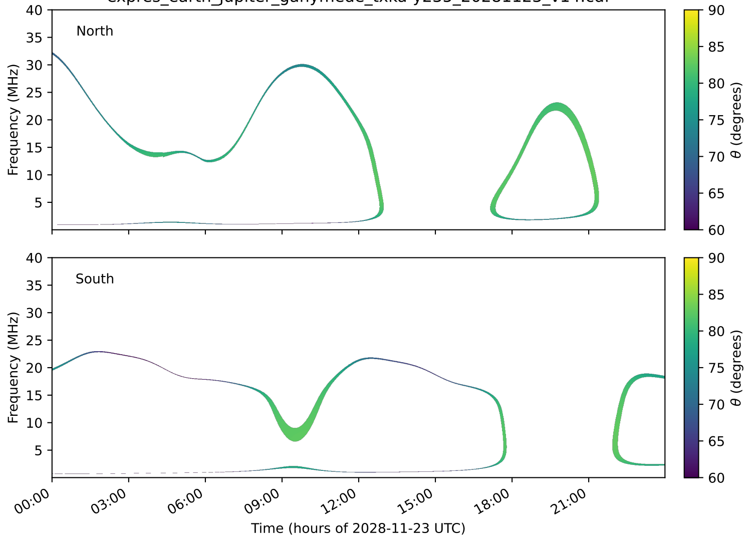
expres_earth_jupiter_ganymede_txka-y235_20281123_v14.cdf
