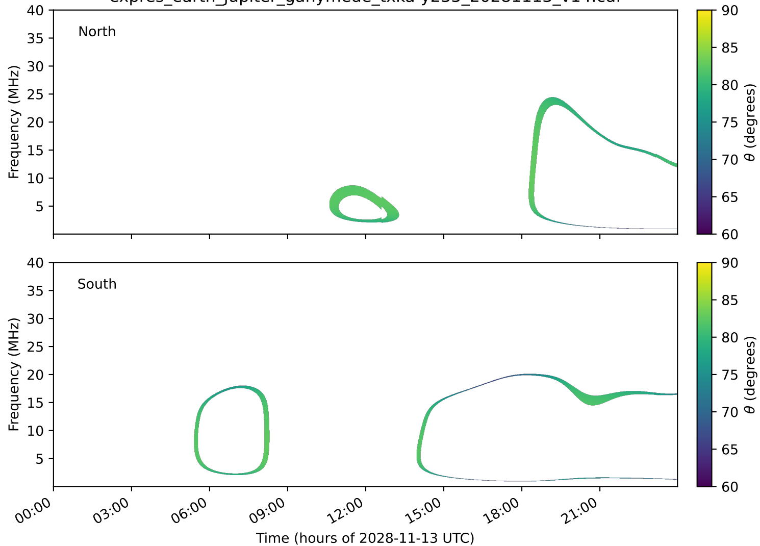
expres_earth_jupiter_ganymede_txka-y235_20281113_v14.cdf
