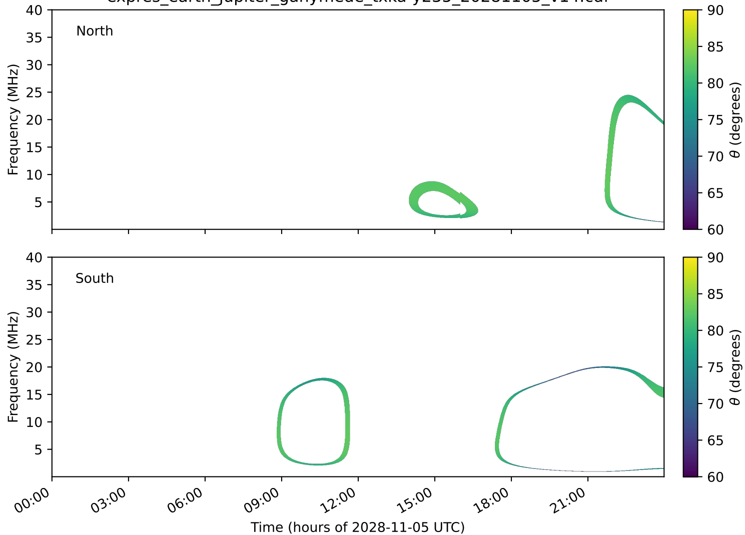
expres_earth_jupiter_ganymede_txka-y235_20281105_v14.cdf
