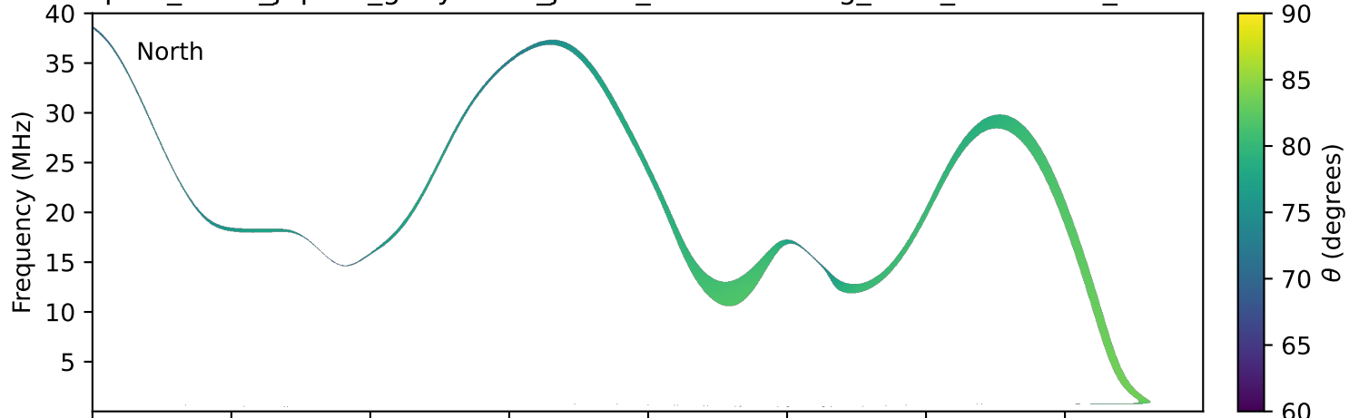
expres_earth_jupiter_ganymede_jrm33_lossc-wid1deg_3kev_20281123_v11.cdf
