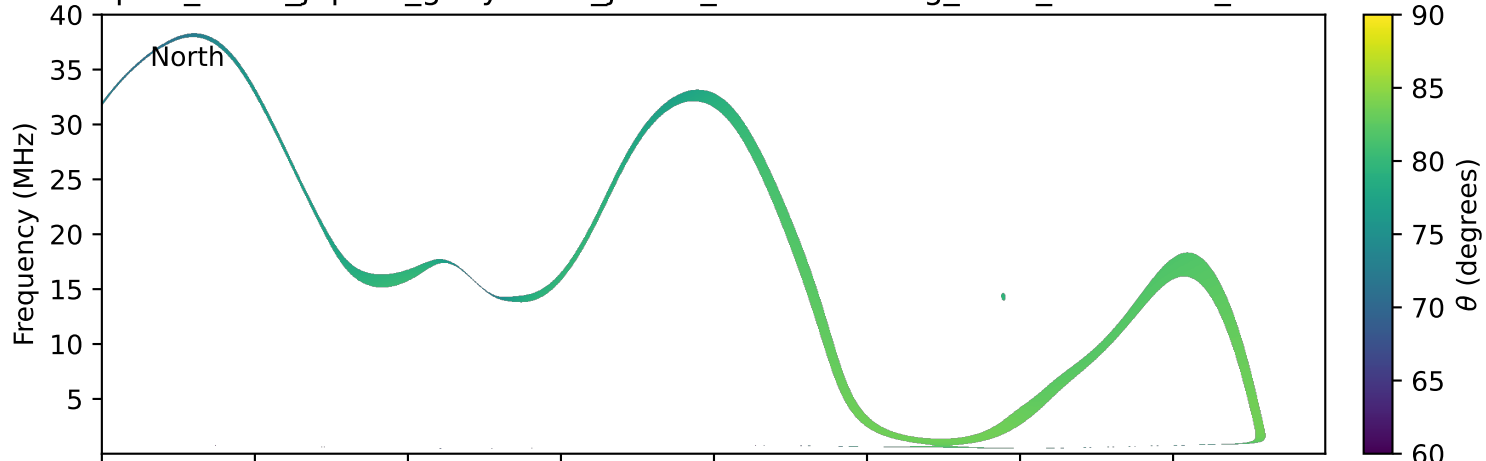
expres_earth_jupiter_ganymede_jrm33_lossc-wid1deg_3kev_20281101_v11.cdf
