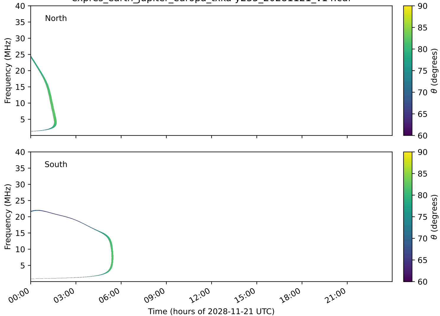
expres_earth_jupiter_europa_txka-y235_20281121_v14.cdf
