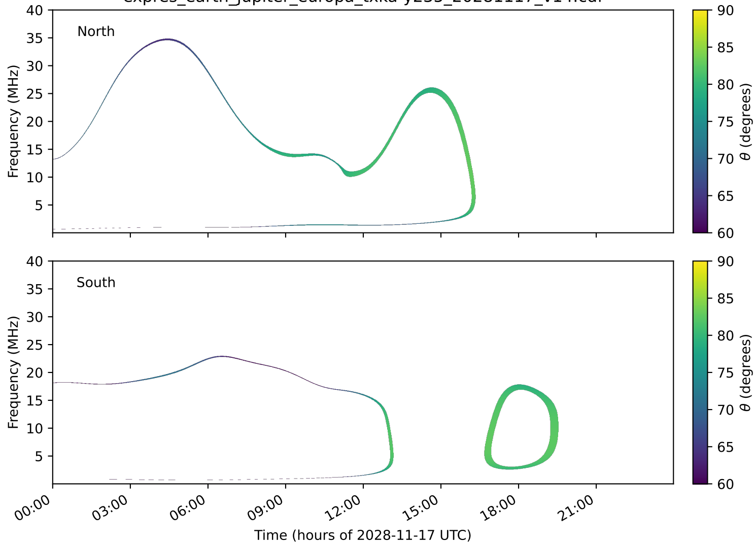
expres_earth_jupiter_europa_txka-y235_20281117_v14.cdf
