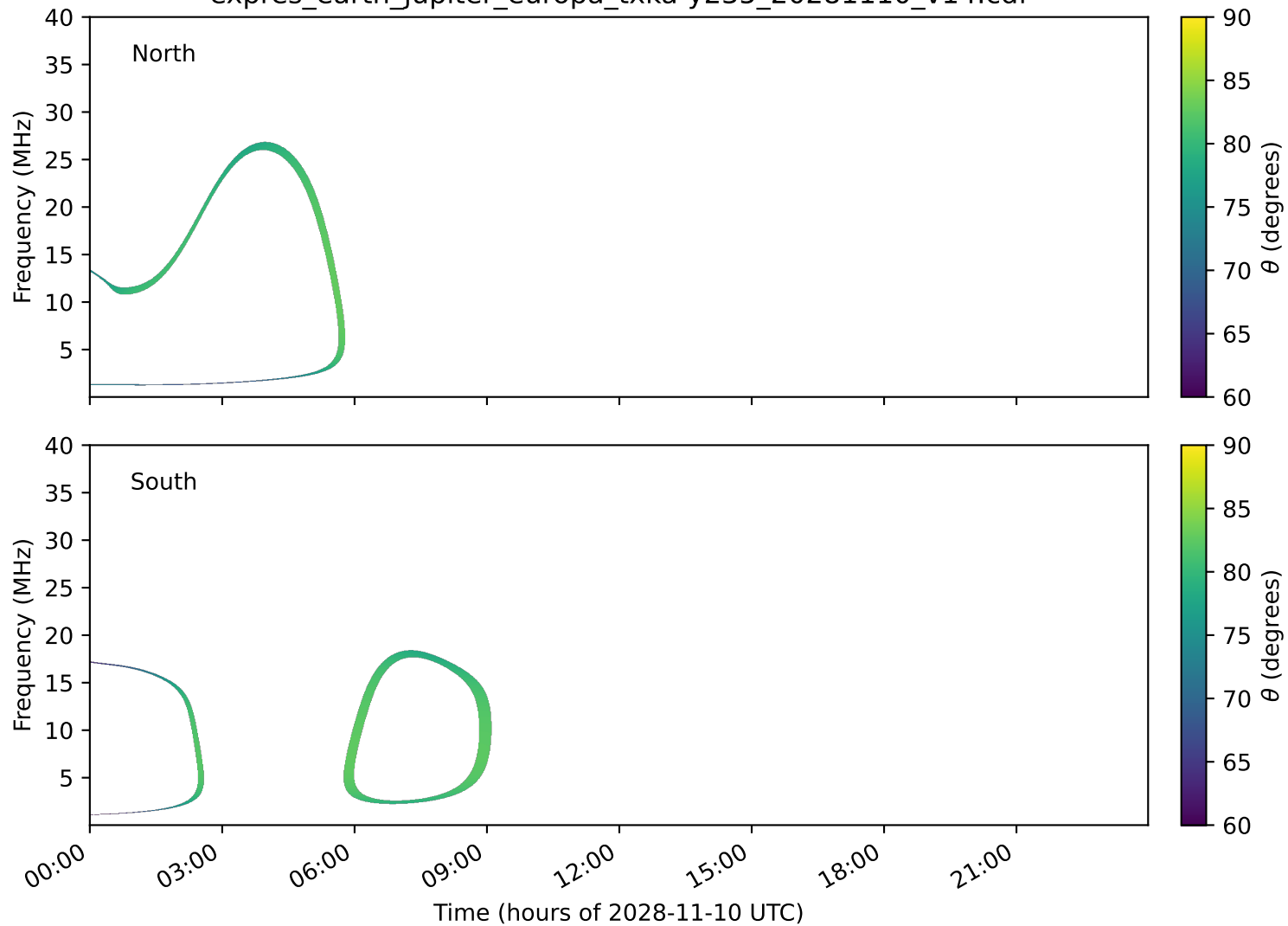
expres_earth_jupiter_europa_txka-y235_20281110_v14.cdf
