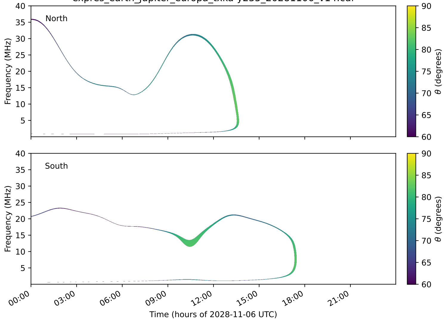
expres_earth_jupiter_europa_txka-y235_20281106_v14.cdf
