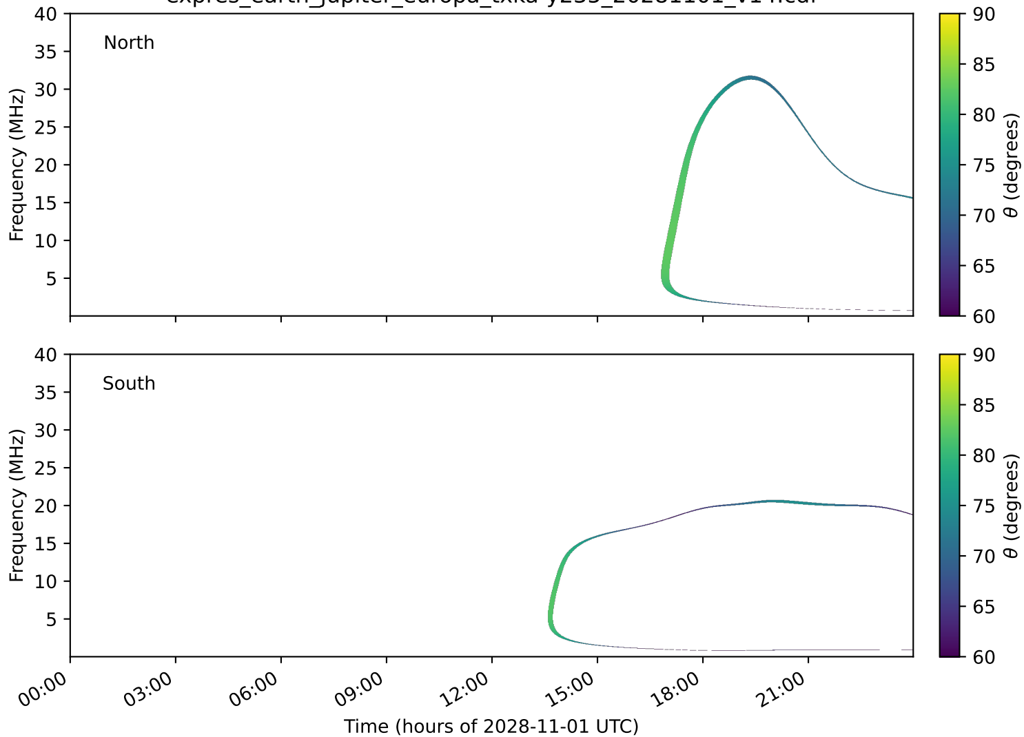
expres_earth_jupiter_europa_txka-y235_20281101_v14.cdf
