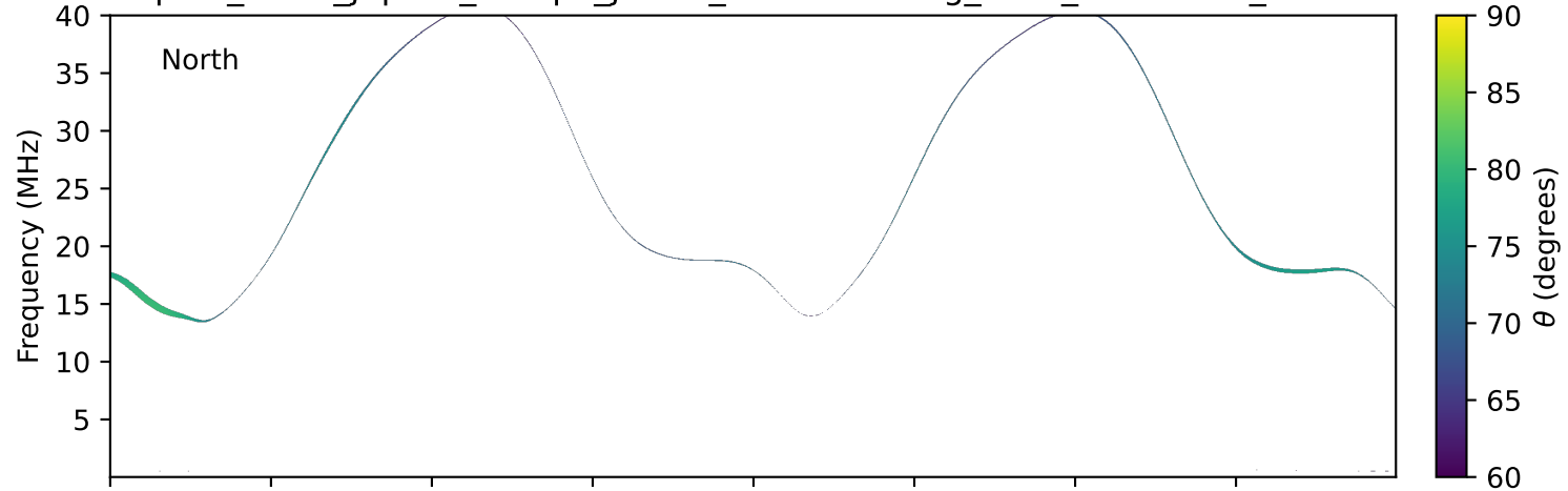
expres_earth_jupiter_europa_jrm33_lossc-wid1deg_3kev_20281109_v11.cdf
