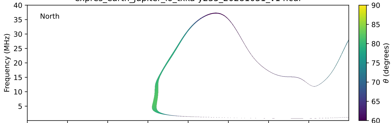
expres_earth_jupiter_io_txka-y235_20281031_v14.cdf
