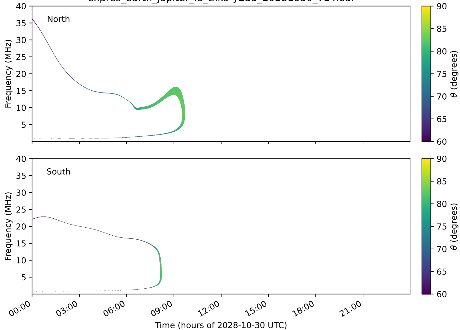
expres_earth_jupiter_io_txka-y235_20281030_v14.cdf
