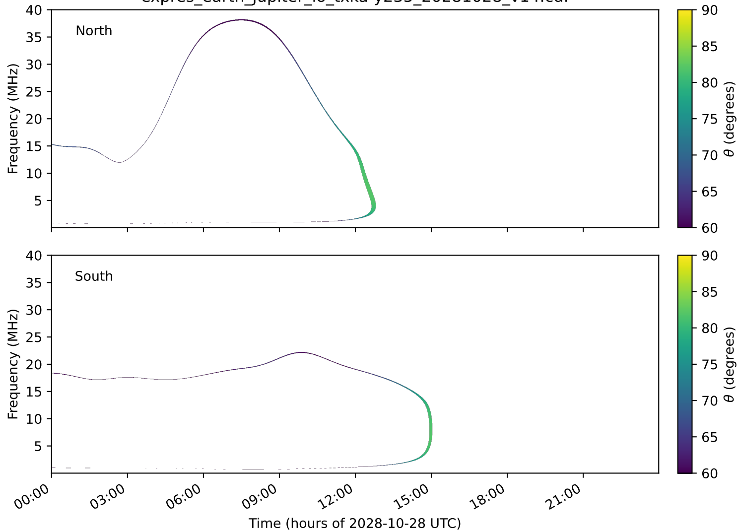
expres_earth_jupiter_io_txka-y235_20281028_v14.cdf
