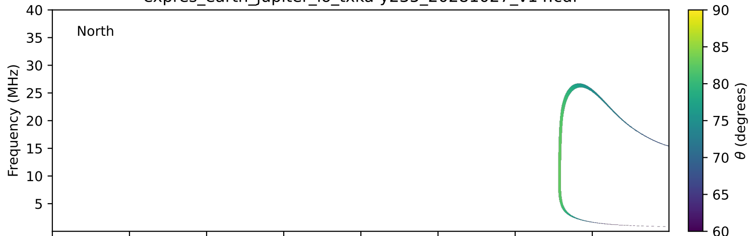
expres_earth_jupiter_io_txka-y235_20281027_v14.cdf
