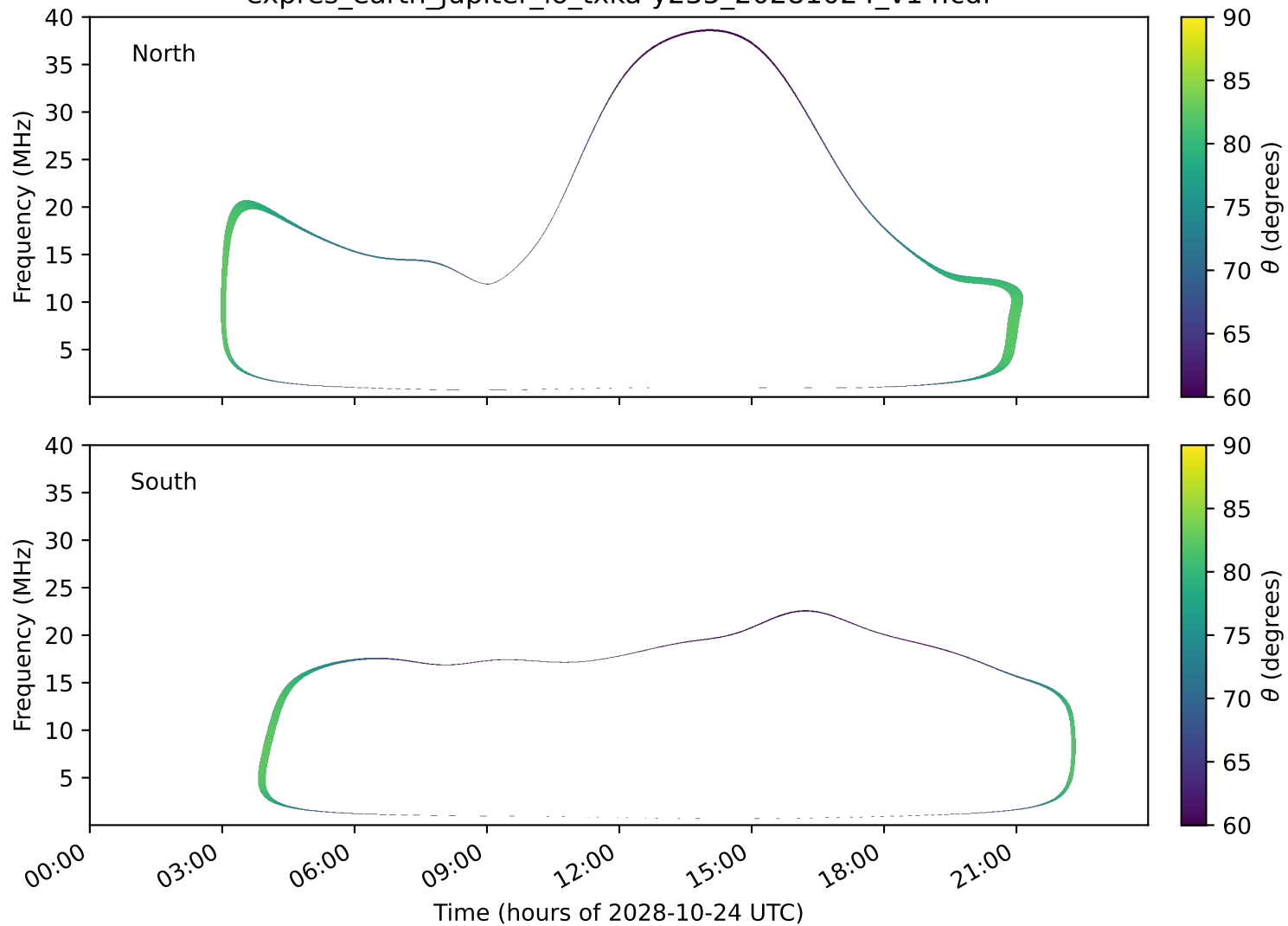
expres_earth_jupiter_io_txka-y235_20281024_v14.cdf
