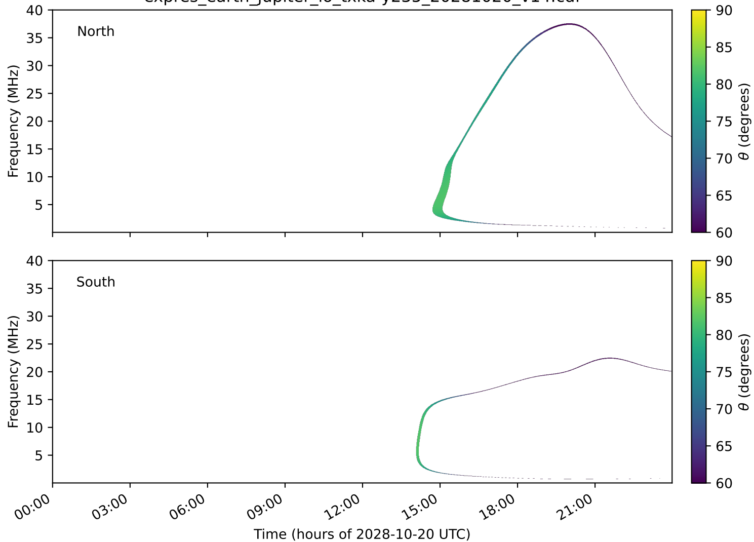
expres_earth_jupiter_io_txka-y235_20281020_v14.cdf
