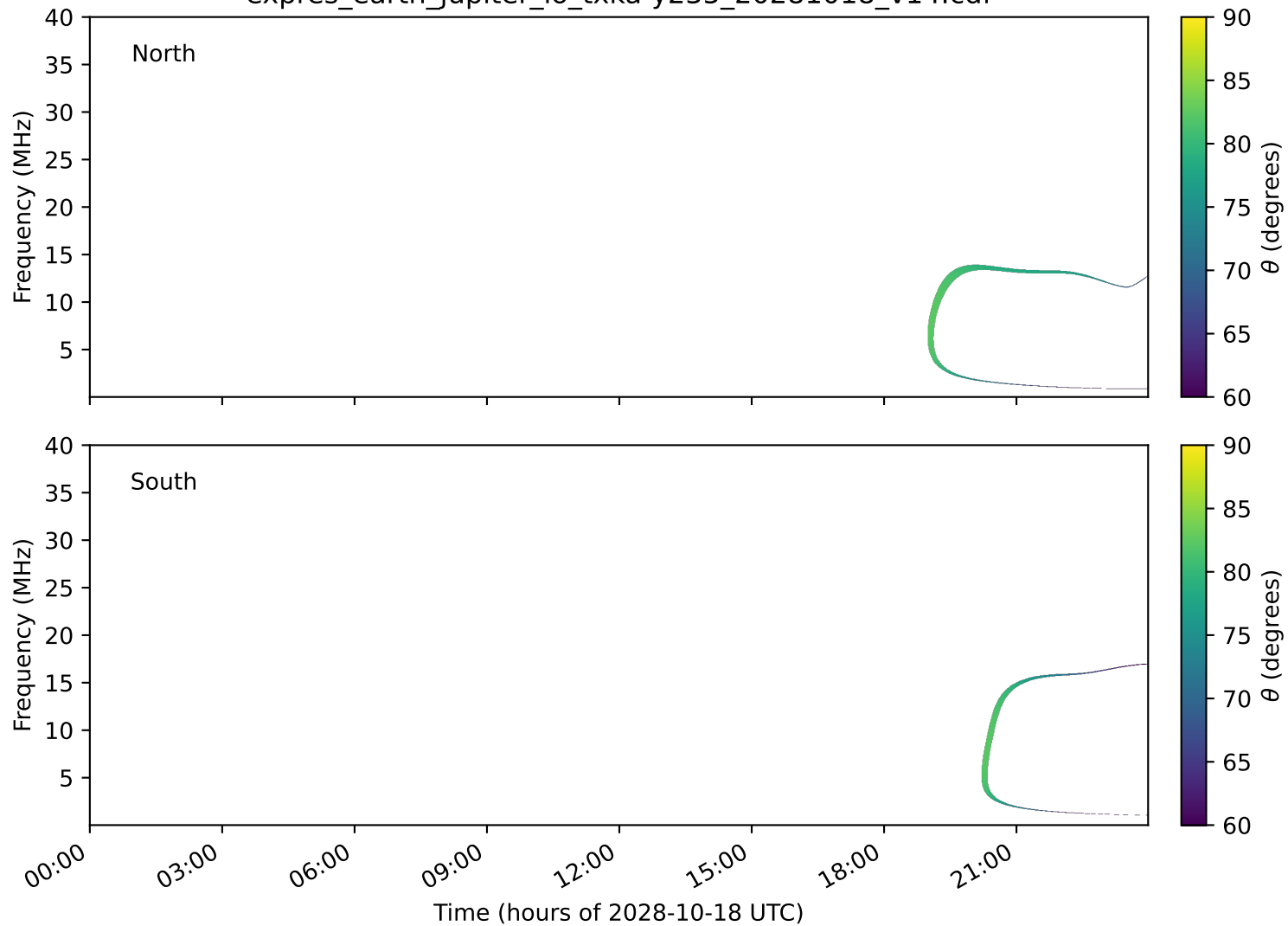
expres_earth_jupiter_io_txka-y235_20281018_v14.cdf
