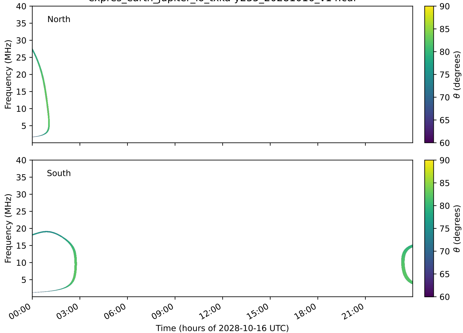
expres_earth_jupiter_io_txka-y235_20281016_v14.cdf
