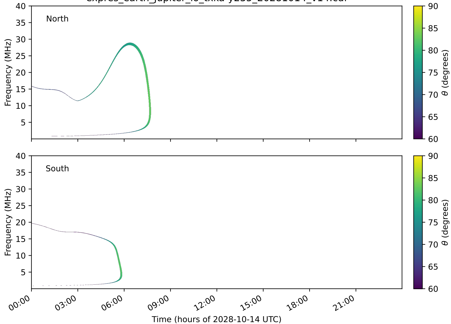
expres_earth_jupiter_io_txka-y235_20281014_v14.cdf
