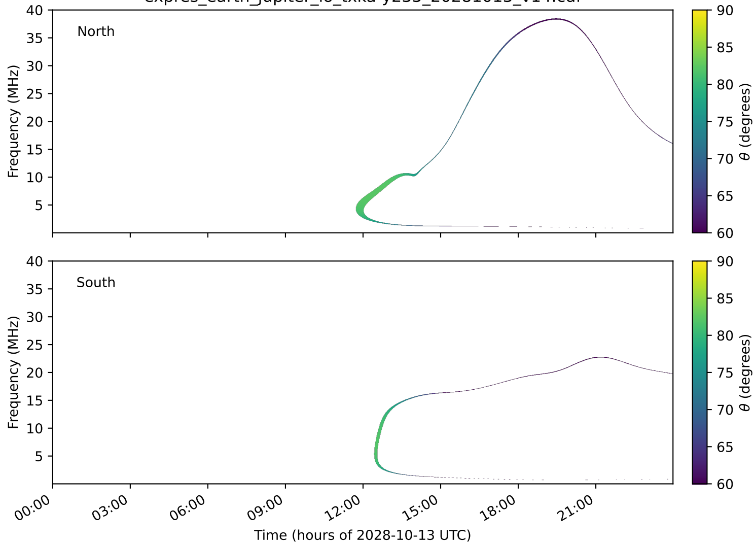
expres_earth_jupiter_io_txka-y235_20281013_v14.cdf
