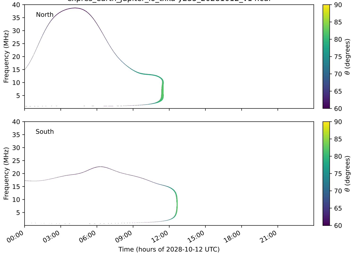
expres_earth_jupiter_io_txka-y235_20281012_v14.cdf
