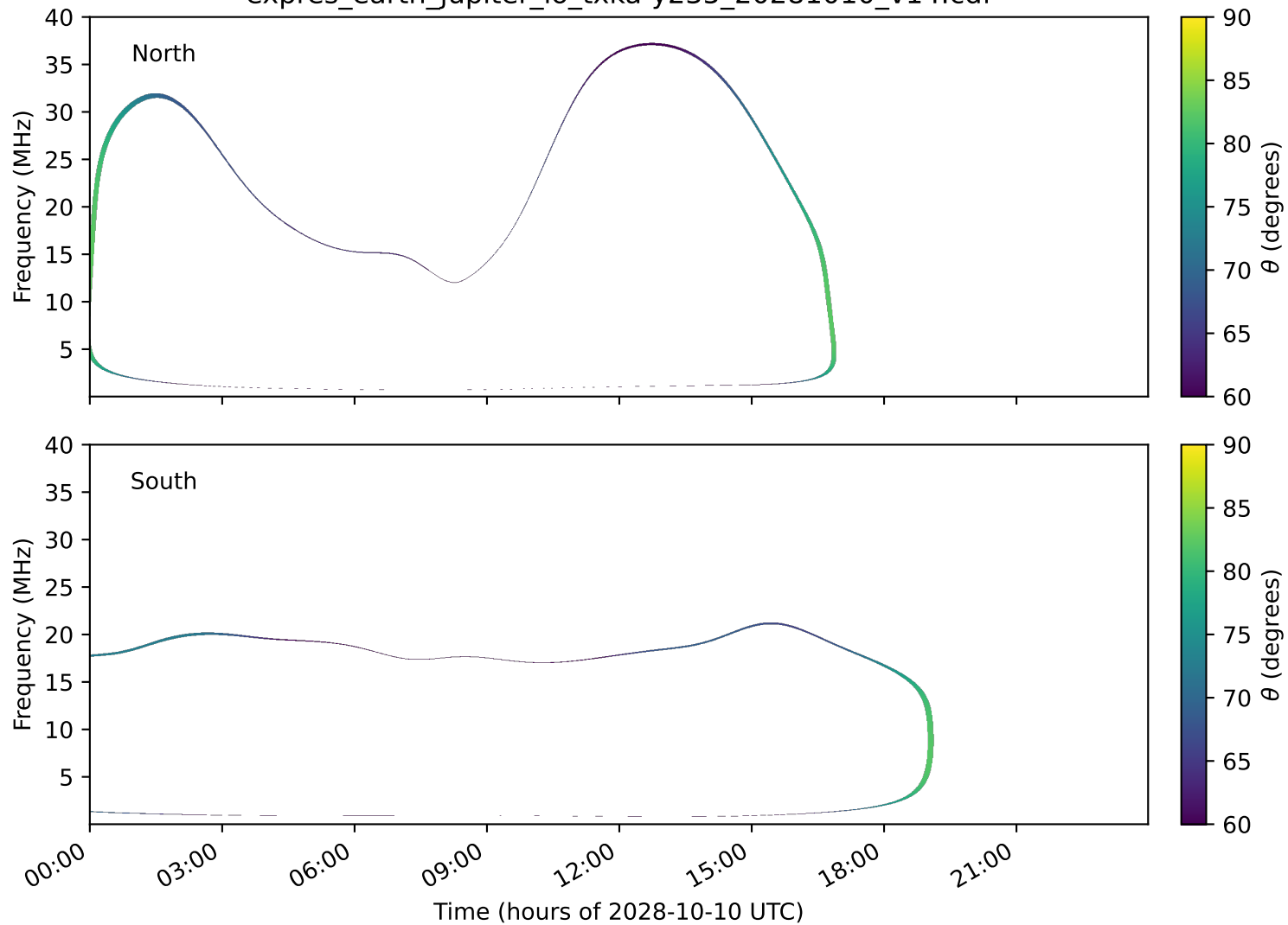
expres_earth_jupiter_io_txka-y235_20281010_v14.cdf
