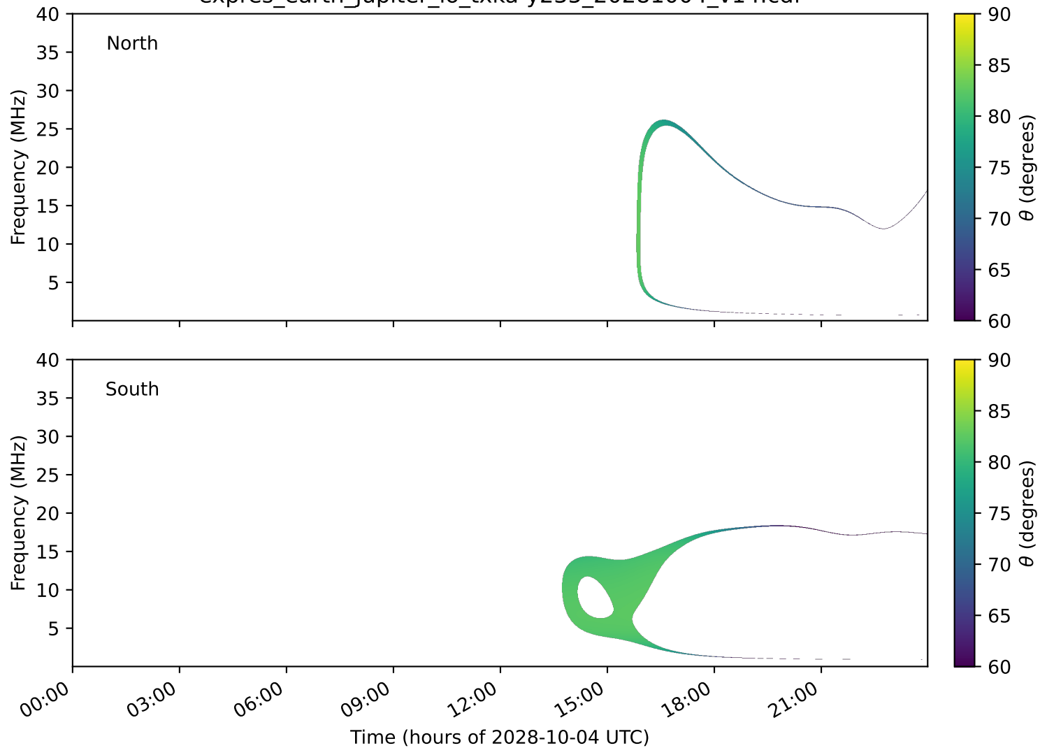
expres_earth_jupiter_io_txka-y235_20281004_v14.cdf
