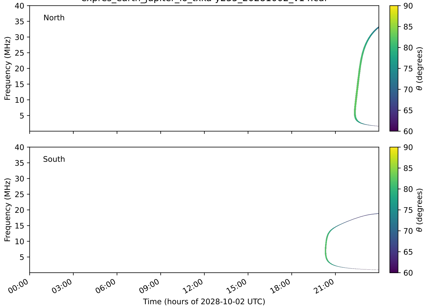
expres_earth_jupiter_io_txka-y235_20281002_v14.cdf
