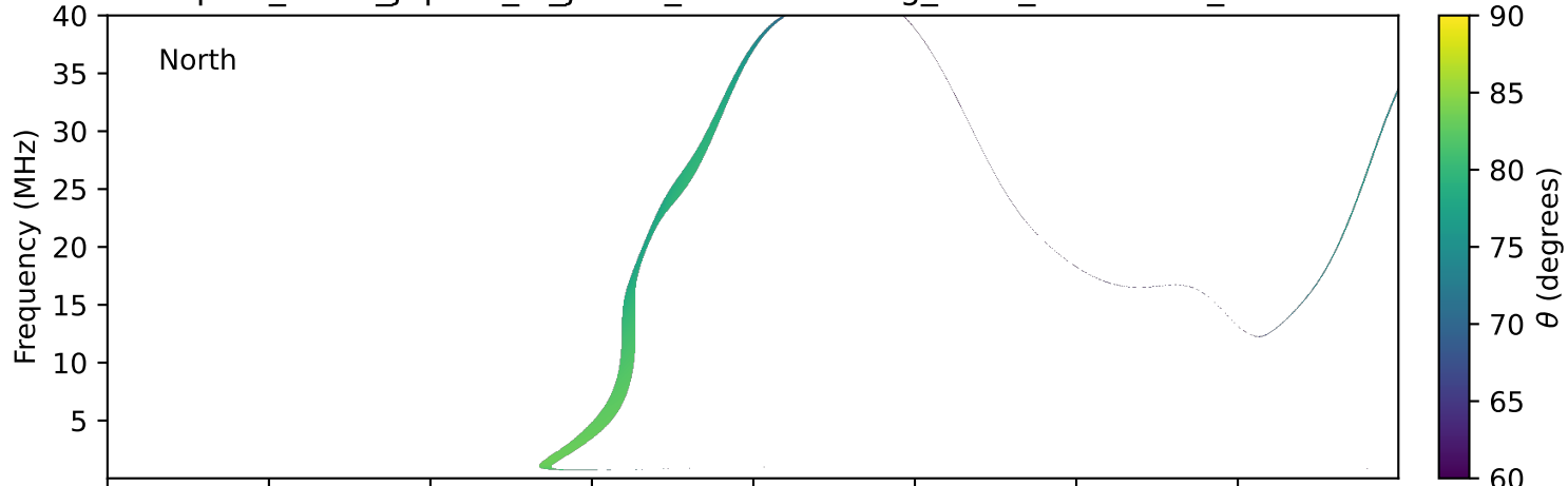
expres_earth_jupiter_io_jrm33_lossc-wid1deg_3kev_20281031_v11.cdf
