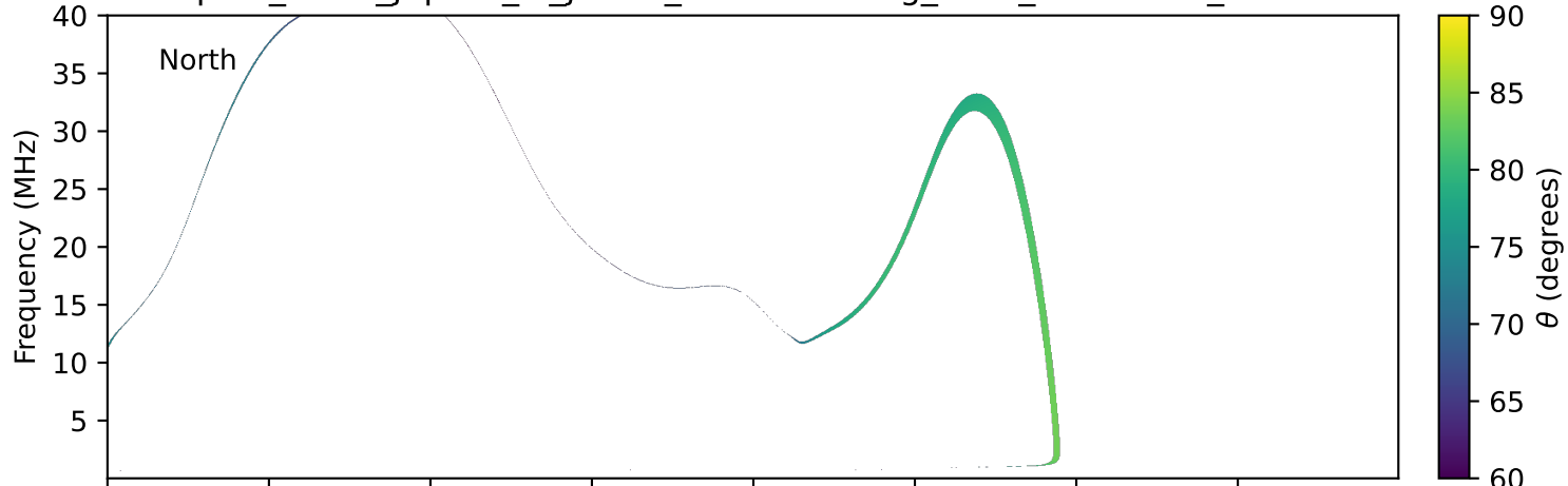
expres_earth_jupiter_io_jrm33_lossc-wid1deg_3kev_20281026_v11.cdf
