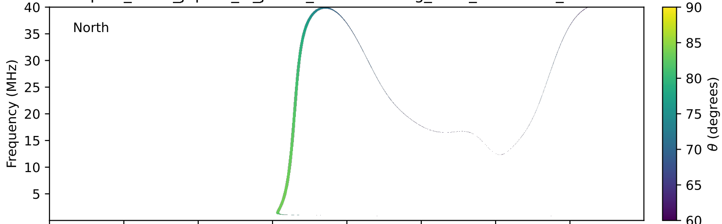
expres_earth_jupiter_io_jrm33_lossc-wid1deg_3kev_20281022_v11.cdf
