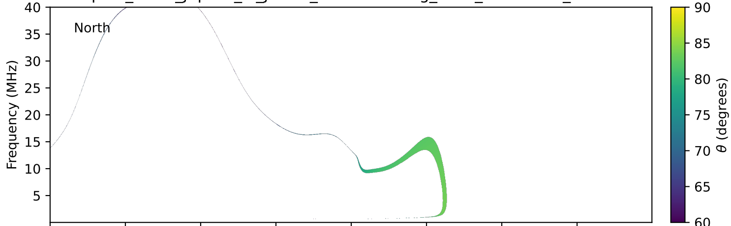
expres_earth_jupiter_io_jrm33_lossc-wid1deg_3kev_20281019_v11.cdf
