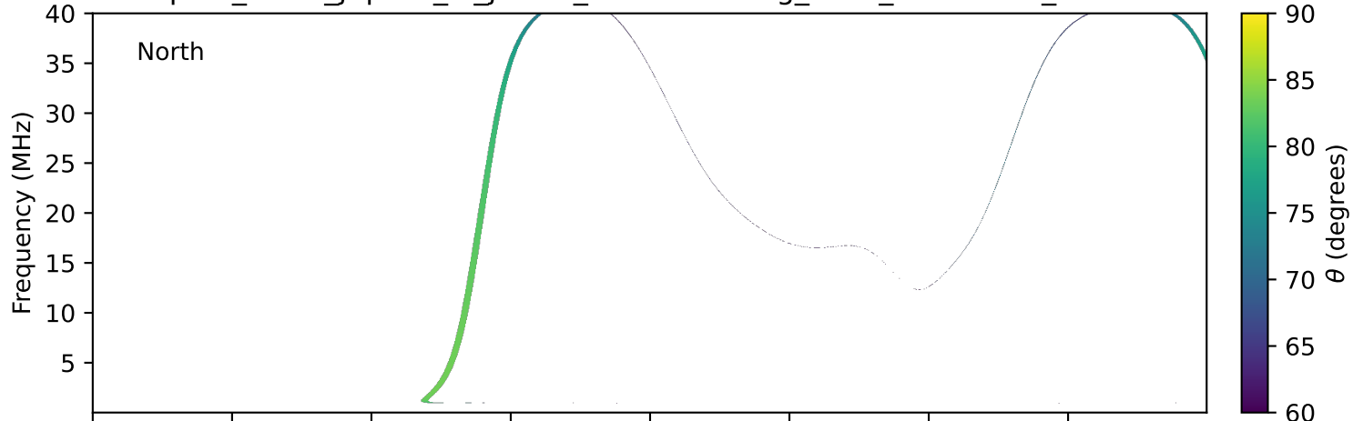
expres_earth_jupiter_io_jrm33_lossc-wid1deg_3kev_20281015_v11.cdf
