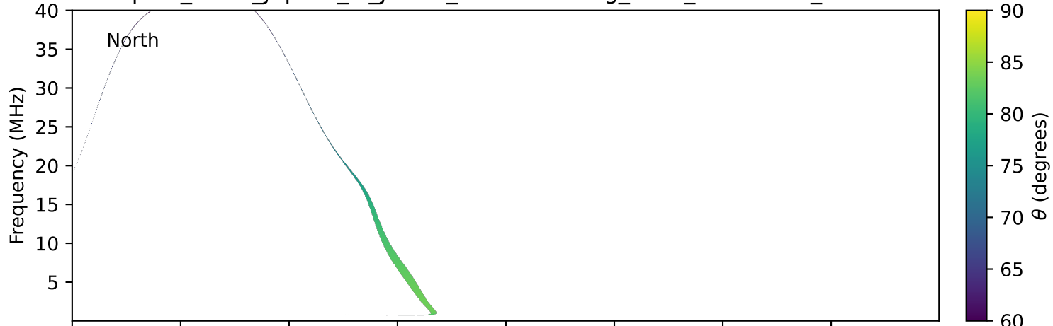
expres_earth_jupiter_io_jrm33_lossc-wid1deg_3kev_20281005_v11.cdf
