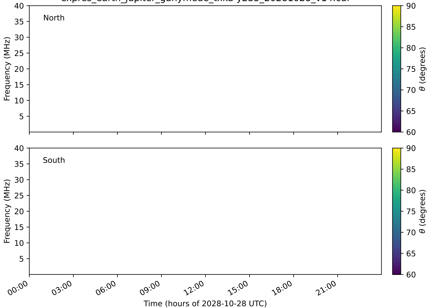
expres_earth_jupiter_ganymede_txka-y235_20281028_v14.cdf
