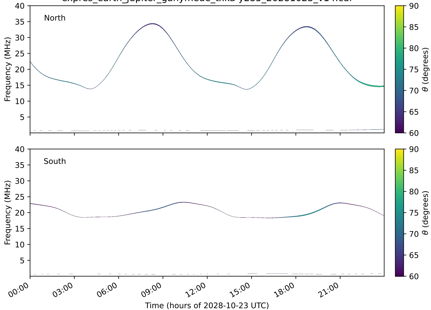
expres_earth_jupiter_ganymede_txka-y235_20281023_v14.cdf
