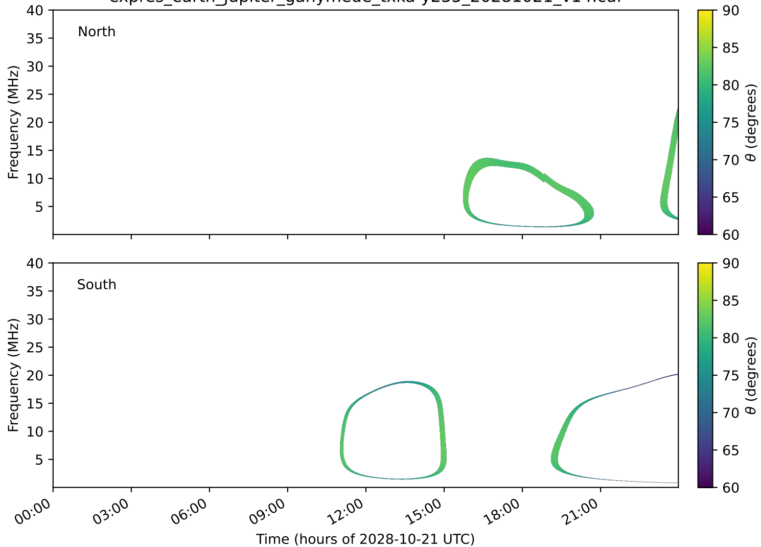
expres_earth_jupiter_ganymede_txka-y235_20281021_v14.cdf
