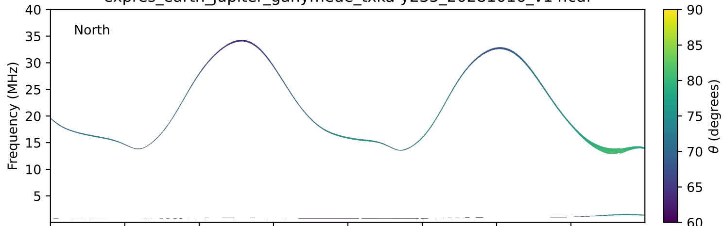
expres_earth_jupiter_ganymede_txka-y235_20281016_v14.cdf
