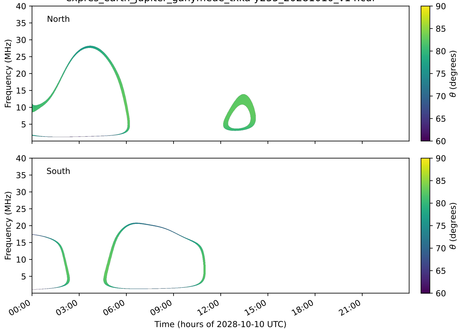
expres_earth_jupiter_ganymede_txka-y235_20281010_v14.cdf
