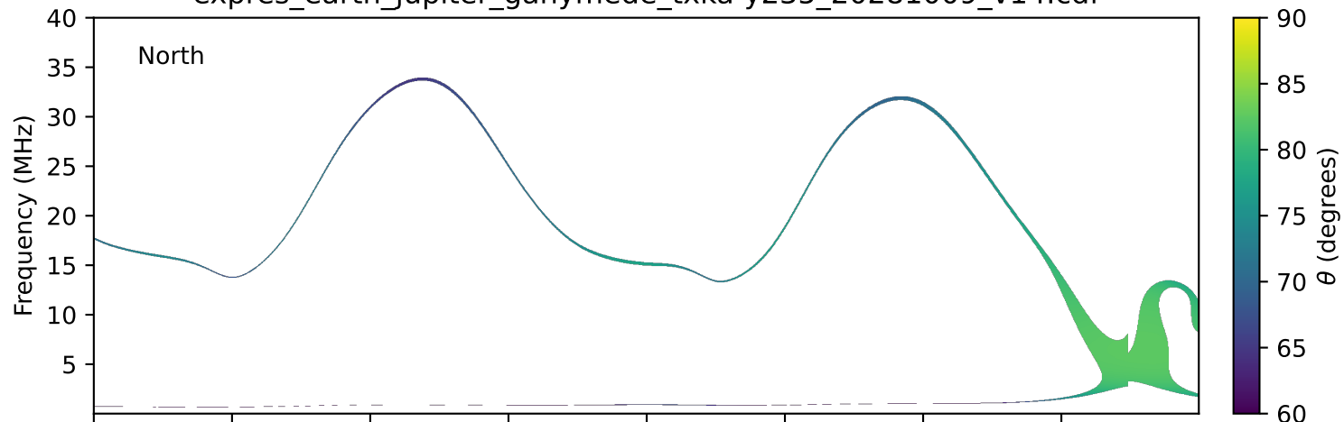
expres_earth_jupiter_ganymede_txka-y235_20281009_v14.cdf
