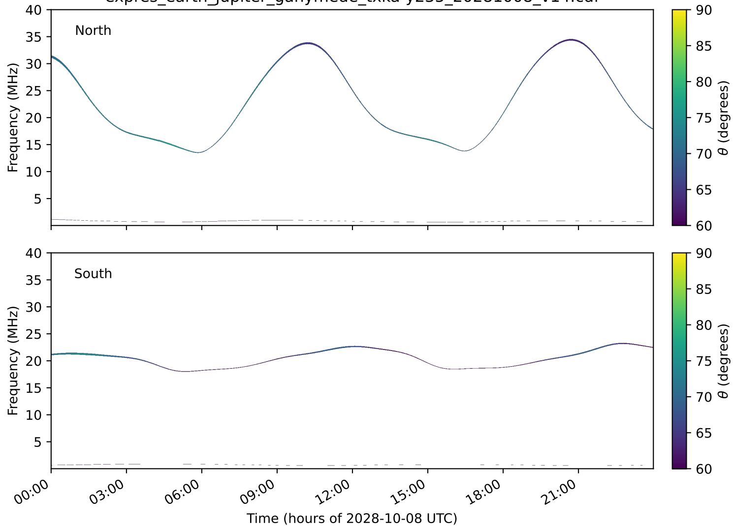
expres_earth_jupiter_ganymede_txka-y235_20281008_v14.cdf
