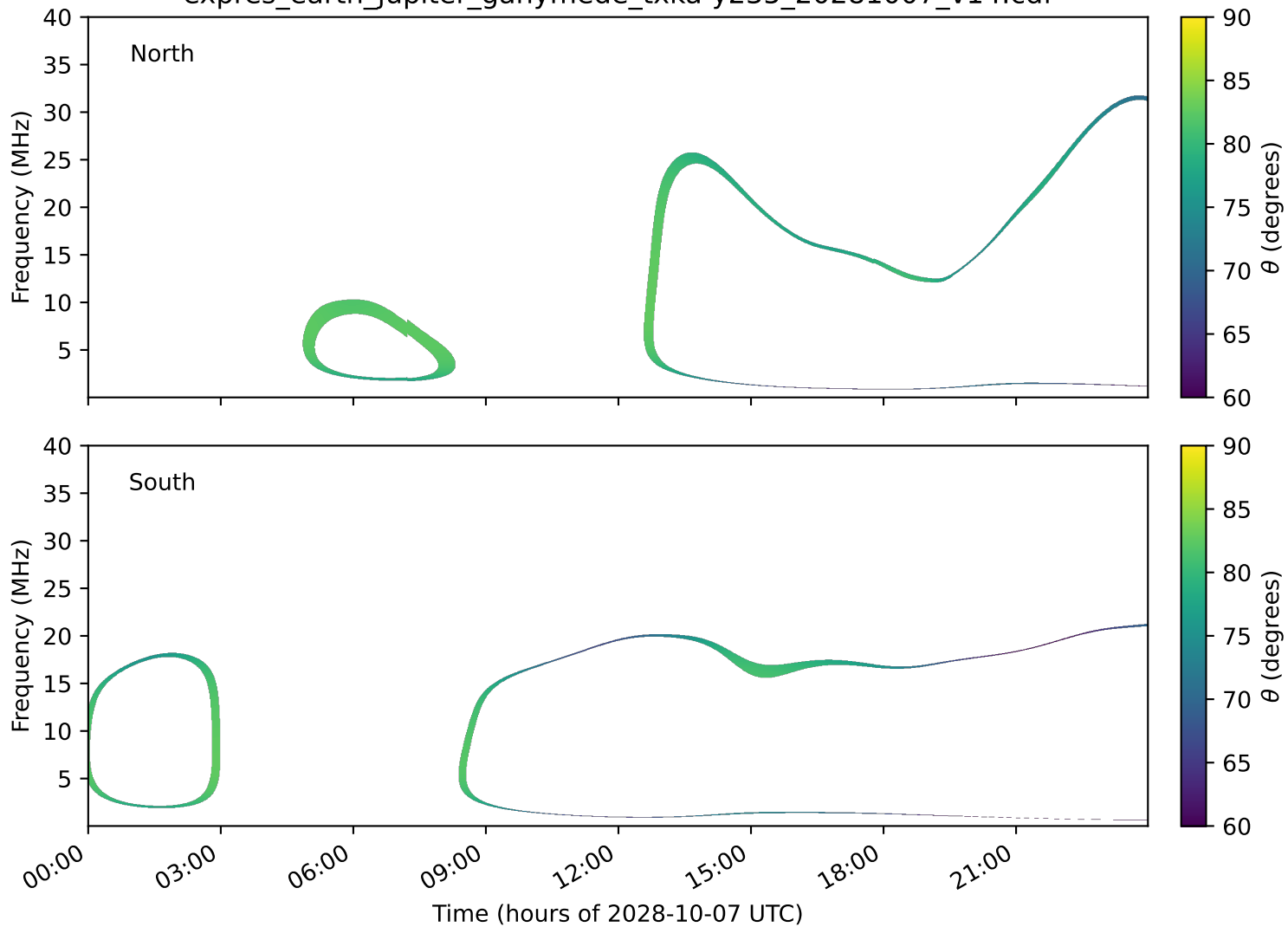
expres_earth_jupiter_ganymede_txka-y235_20281007_v14.cdf
