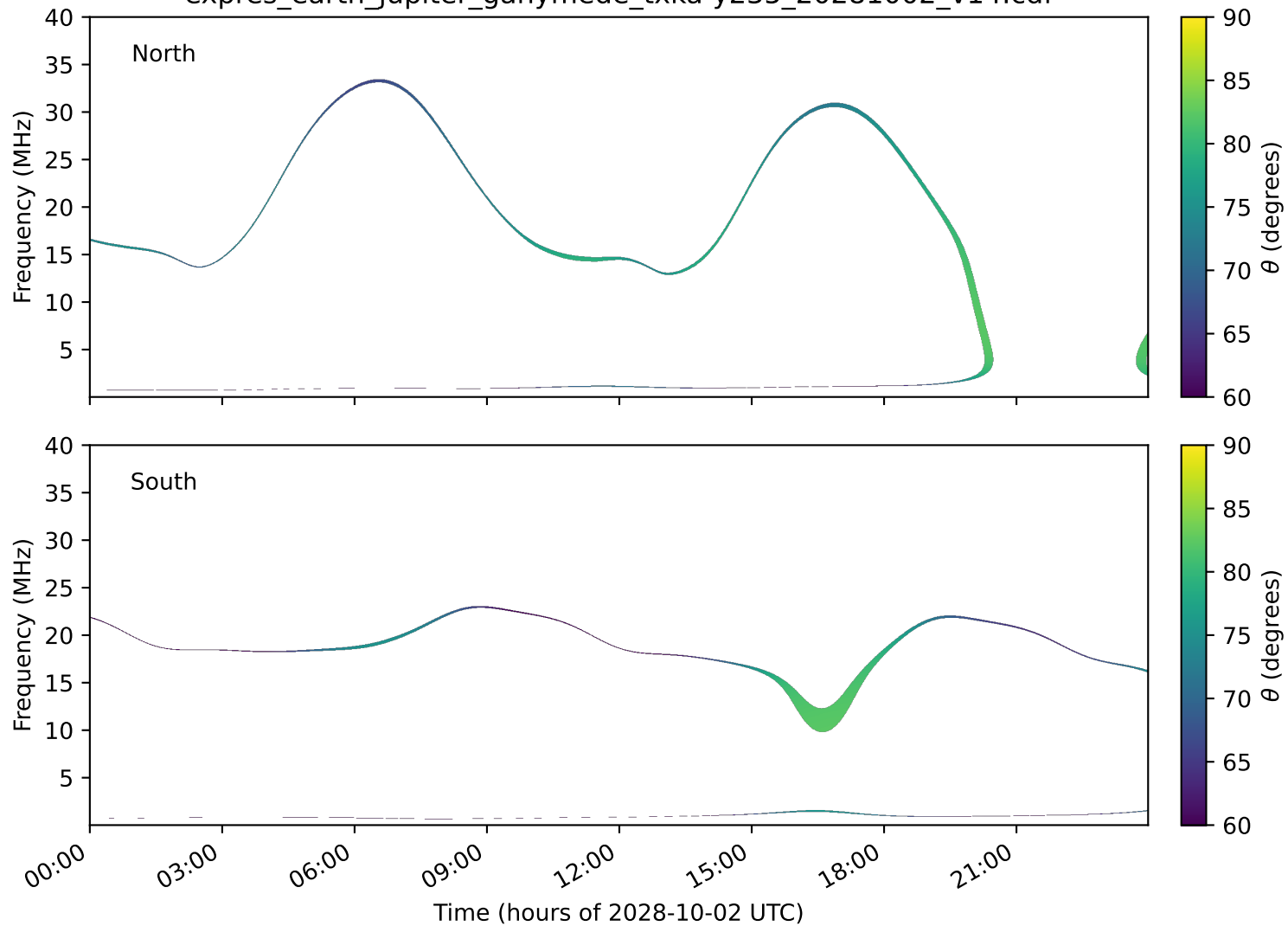
expres_earth_jupiter_ganymede_txka-y235_20281002_v14.cdf
