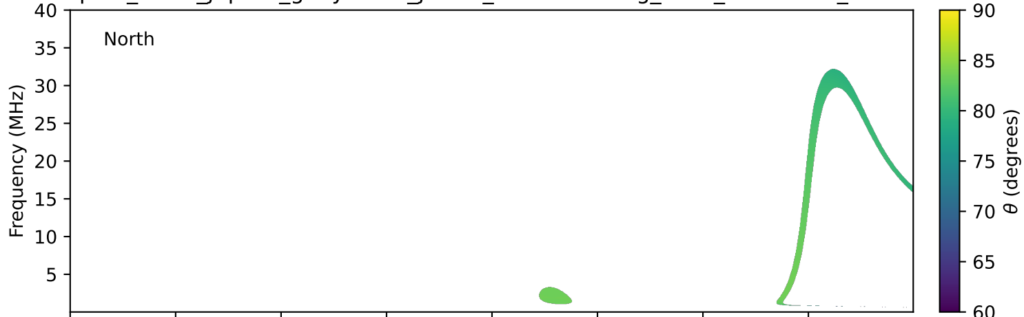
expres_earth_jupiter_ganymede_jrm33_lossc-wid1deg_3kev_20281029_v11.cdf
