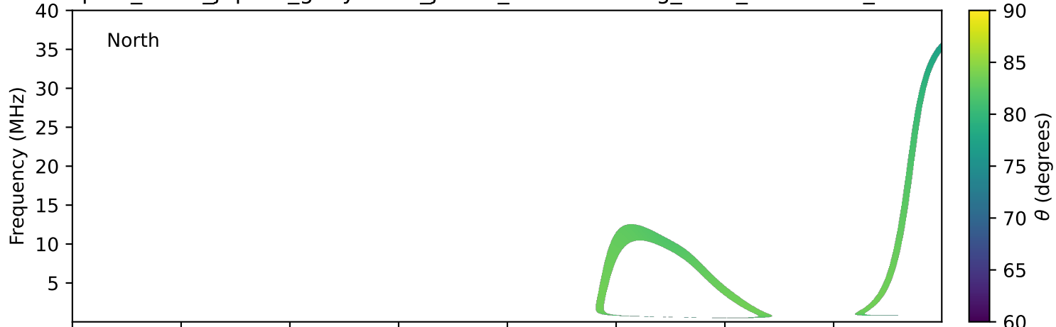
expres_earth_jupiter_ganymede_jrm33_lossc-wid1deg_3kev_20281014_v11.cdf
