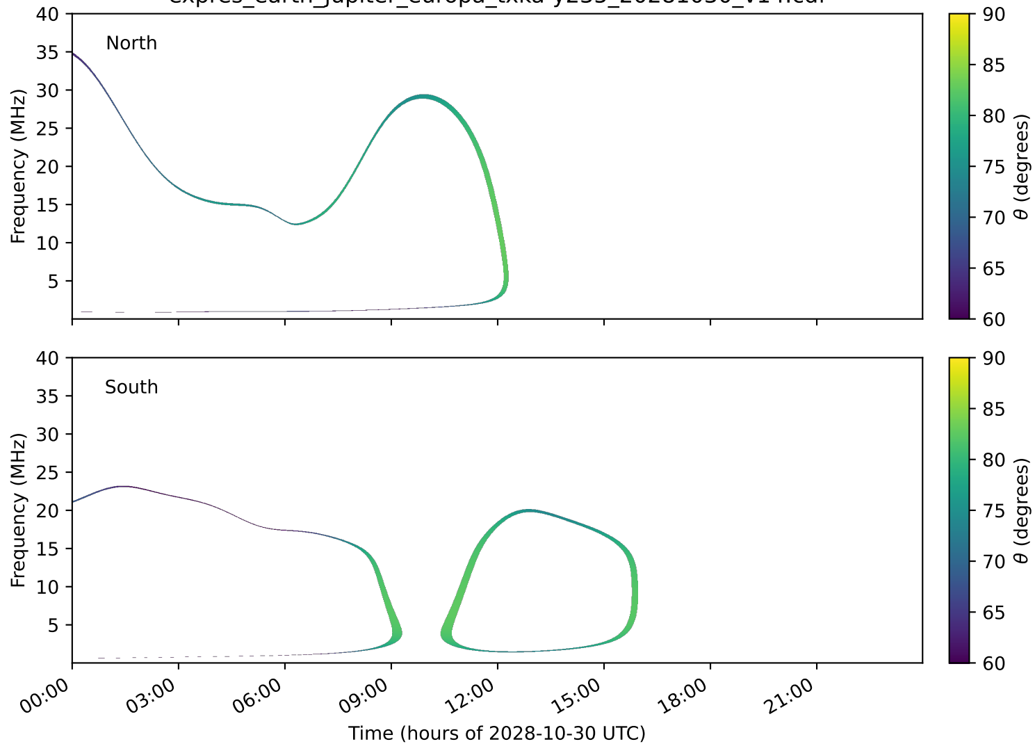
expres_earth_jupiter_europa_txka-y235_20281030_v14.cdf
