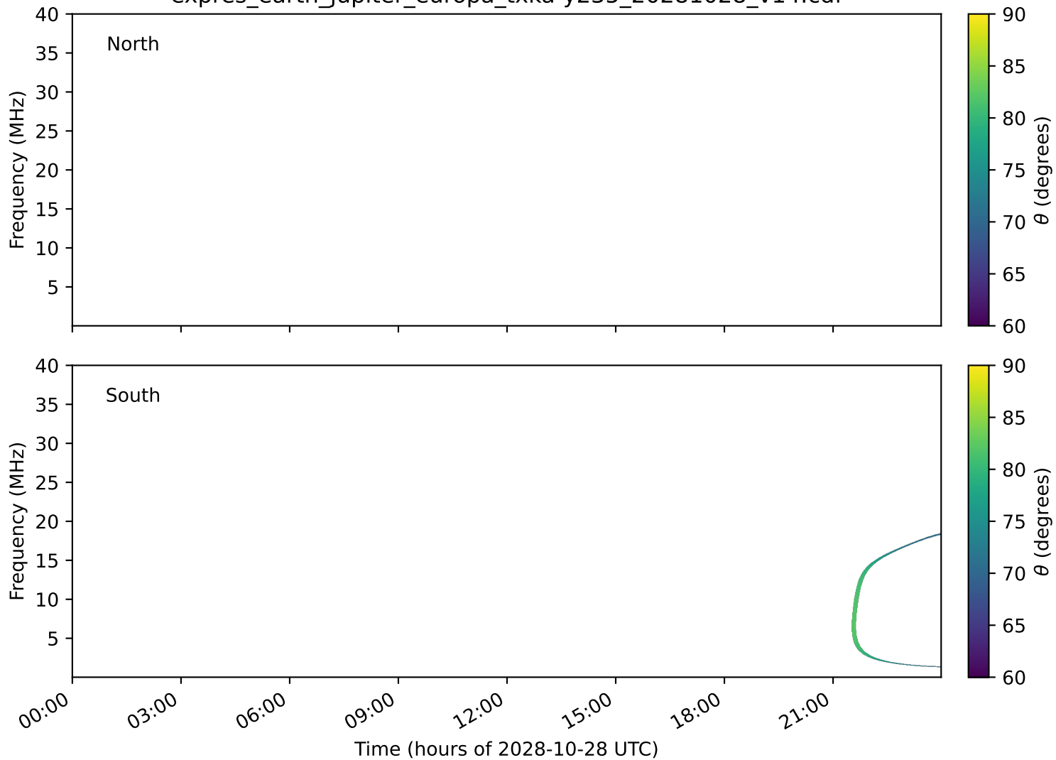
expres_earth_jupiter_europa_txka-y235_20281028_v14.cdf
